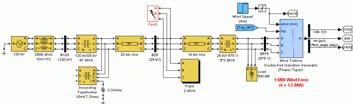
Simscape Power Systems Diagram of the Wind Farm Connected to the Distribution System ( power_wind_dfig )
