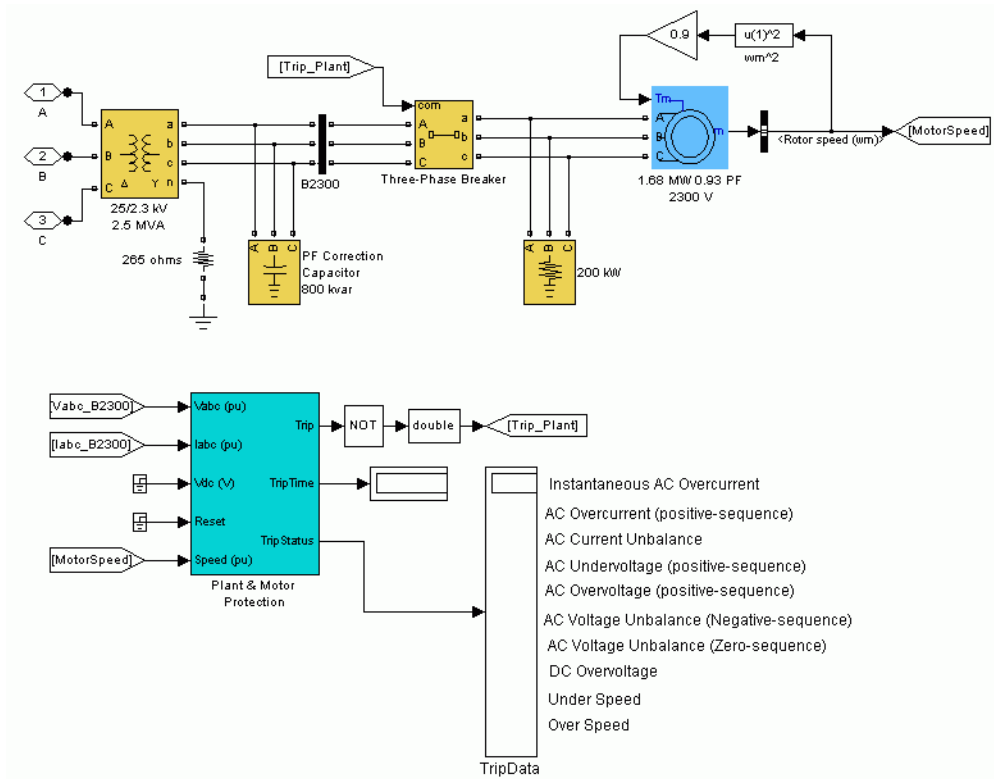
Simscape Power Systems Diagram of the 2 MVA Plant with Its Protection System
